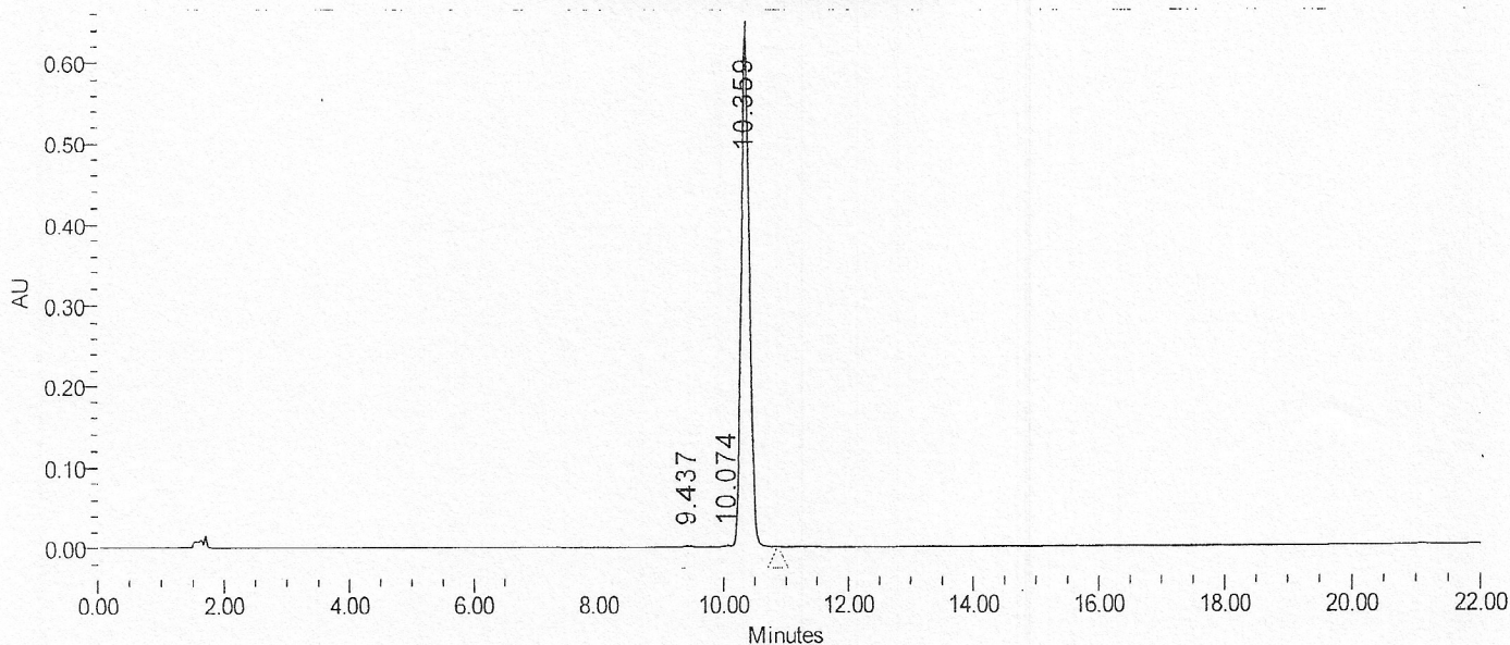
Auto-Scaled Chromatogram
